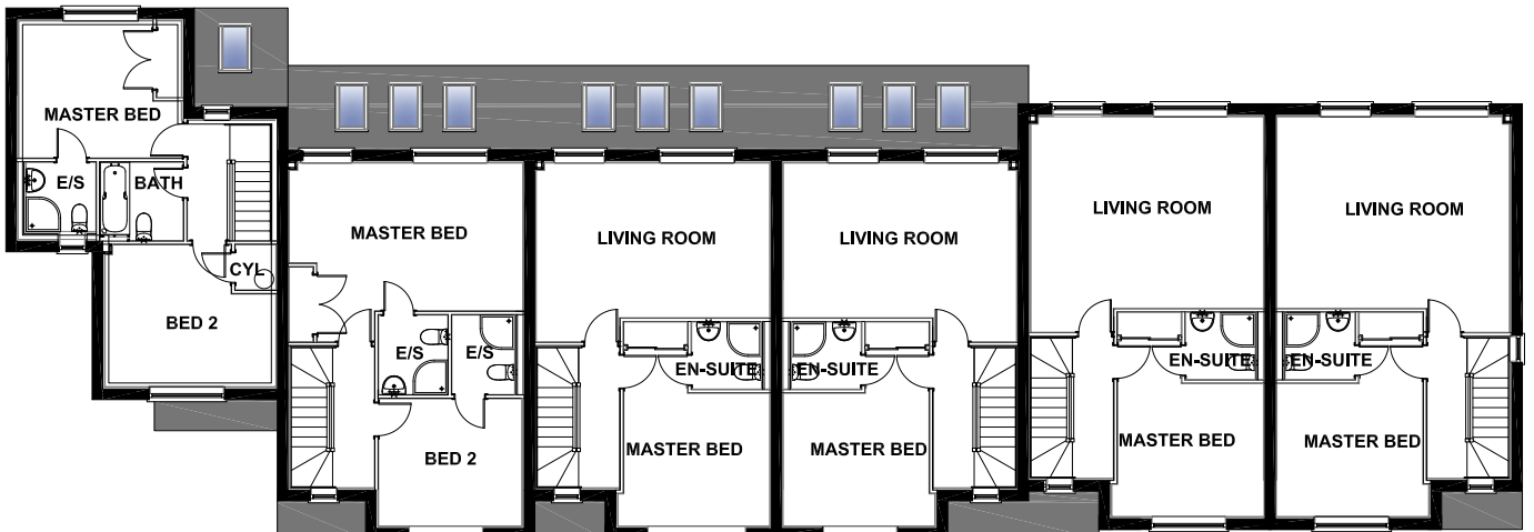
FIRST FLOOR
